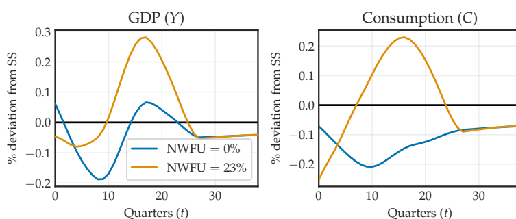
Figure 7: IRFs to a US MP Shock
