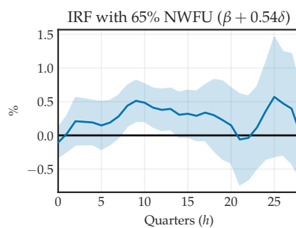
Figure A.10: State-Dependent Local Projections at 2020 NWFU
