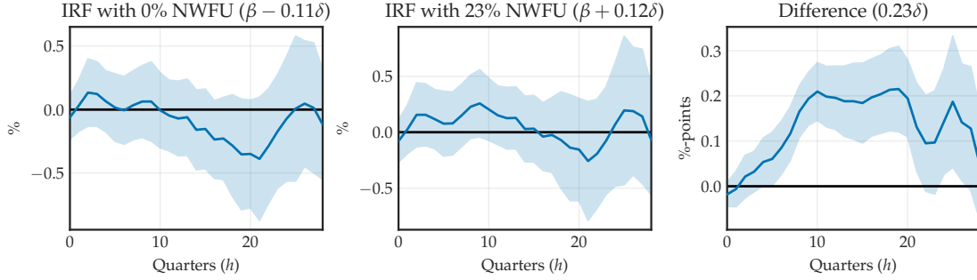
Figure A.6: State-Dependent Local Projections With 4 Lags
