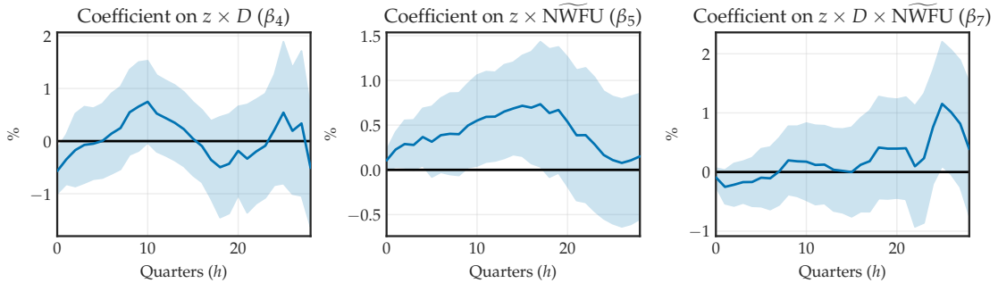
Figure 5: Spillovers of US MP Onto Foreign GDP With NWFU and Time Interactions
