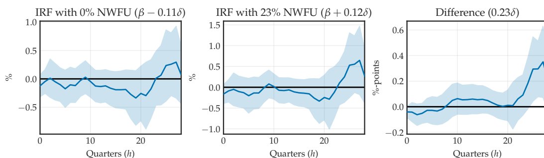
Figure A.9: State-Dependent Local Projections With Consumption
